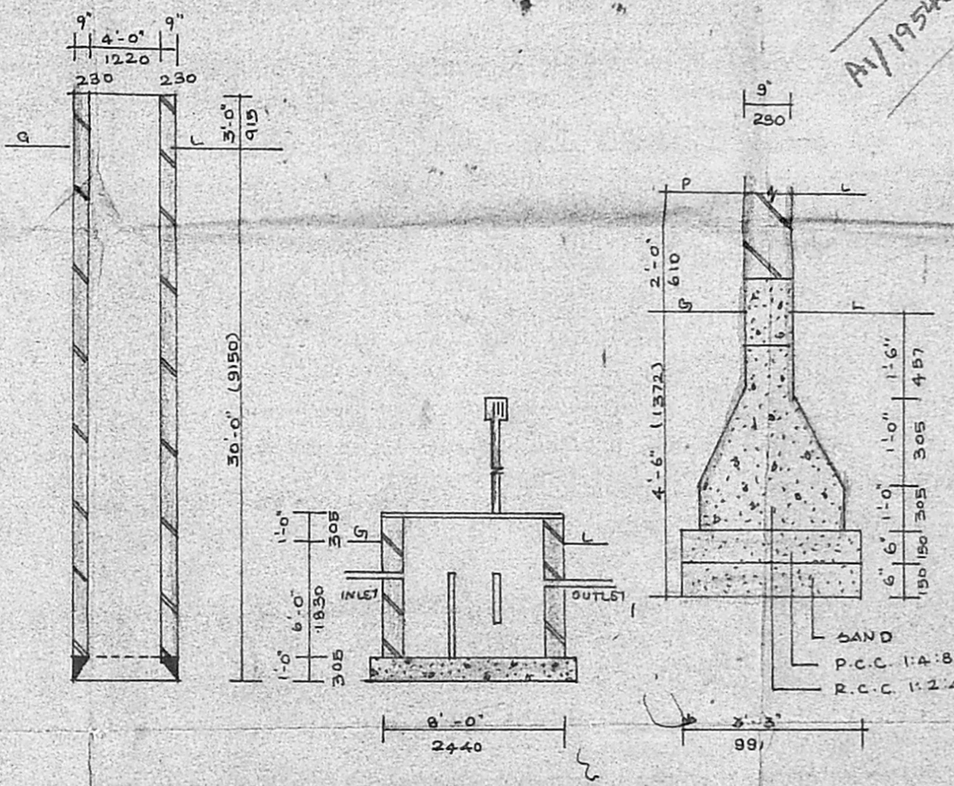
DETAILS OF WELL SEPTIC TANK AND COLUMN
